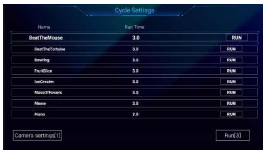
main interface
